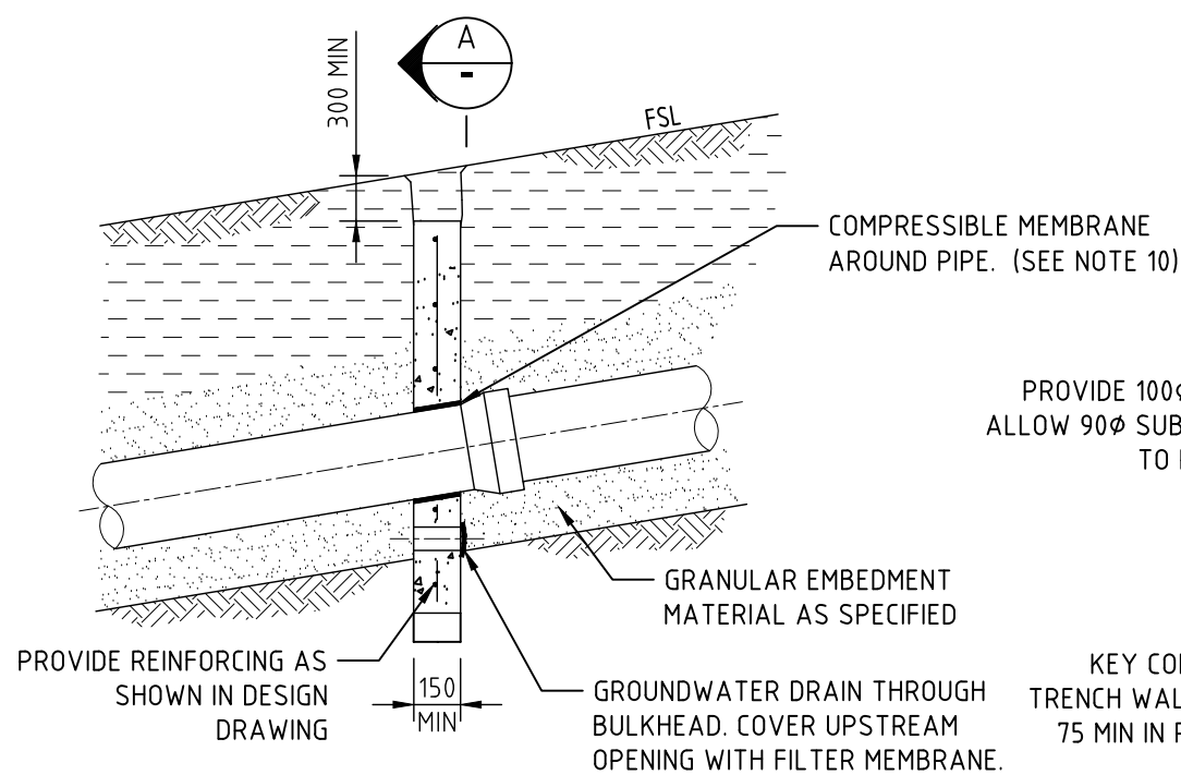
CONCRETE BULKHEAD DETAIL
