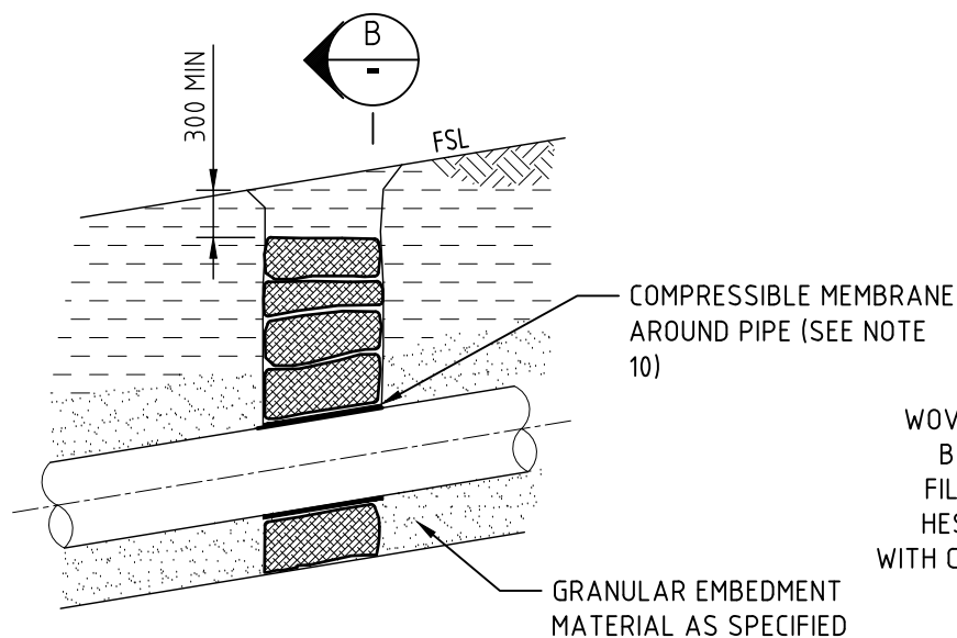
TRENCH STOP DETAIL
