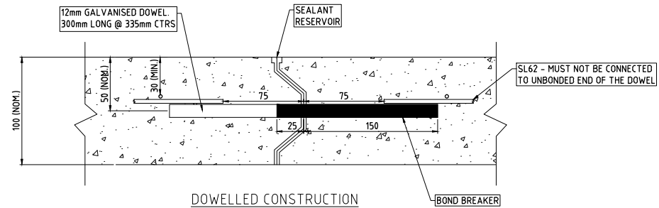
DOWELLED CONSTRUCTION (CONNOLLY) JOINT - REINFORCED
