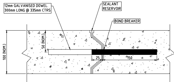
DOWELLED CONSTRUCTION (CONNOLLY) JOINT - UNREINFORCED
