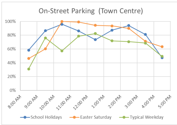
Figure 4-3 Daily Off and On-Street Parking Utilisation Rates – Town Centre
